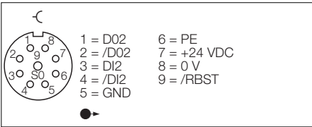
Fieldbus output (M23)
