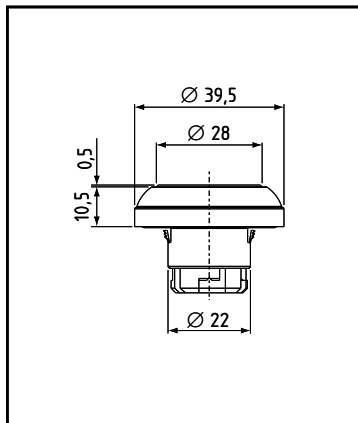
Pushbutton Ex-RDT ..
